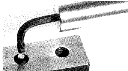
Twisted to about 270°, the key shears off clean. Note the extension bar illustrated for test purposes only.
